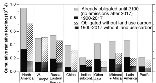
Fig. 2. The cumulative contributions to global mean net RF by emissions from the nine regions of the world. The dark bars on the left side for each region are the cumulative RF to date due to emissions from 1900 to 2017. The gray bars above the dark bars are what would be retained by 2100 due to emissions to date, i.e., what the world has already committed to because of GHGs that are already in the atmosphere. The hatched bars to the right are the same quantities without land-use carbon changes.
